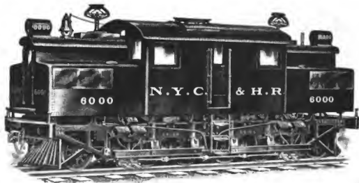
New York Central Type 4 Electric Locomotive. Direct Current—100 tons—2200 horse-power—80 m. p. h. Built by General Electric Company and American Locomotive Company.
